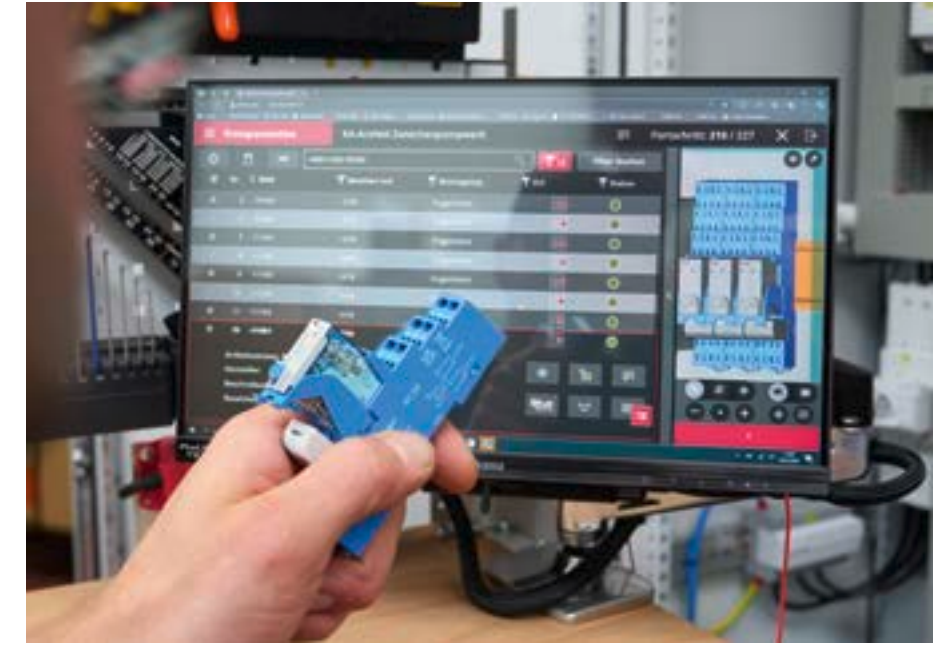
Eplan Pro Panel is used to create the enclosure's digital twin, which then provides the basis for manufacturing with Smart Mounting.
