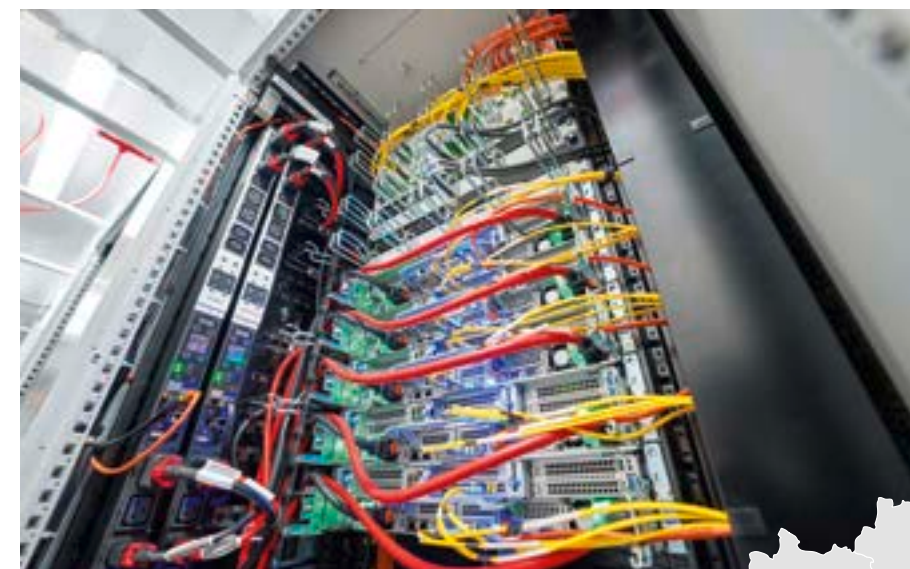
Everything in colourful order – a peek inside one of the Rittal VX IT server racks at BORA.
